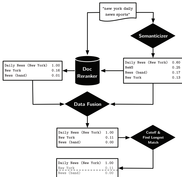
Figure 1: A schematic view of our system pipeline. A query is given as input to the Semanticizer for generating a ranked list of candidate entities using several methods. The candidate list is refined using a document re-ranker and then all ranked lists are merged together using late data fusion. The final entities for the query are selected using cutoff on their retrieval score, and longest matches are preferred over shorter ones.
